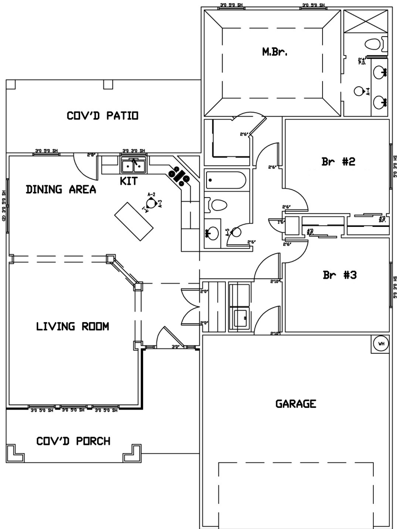
The "Mancini" 1,300 sq. ft. Living Area
